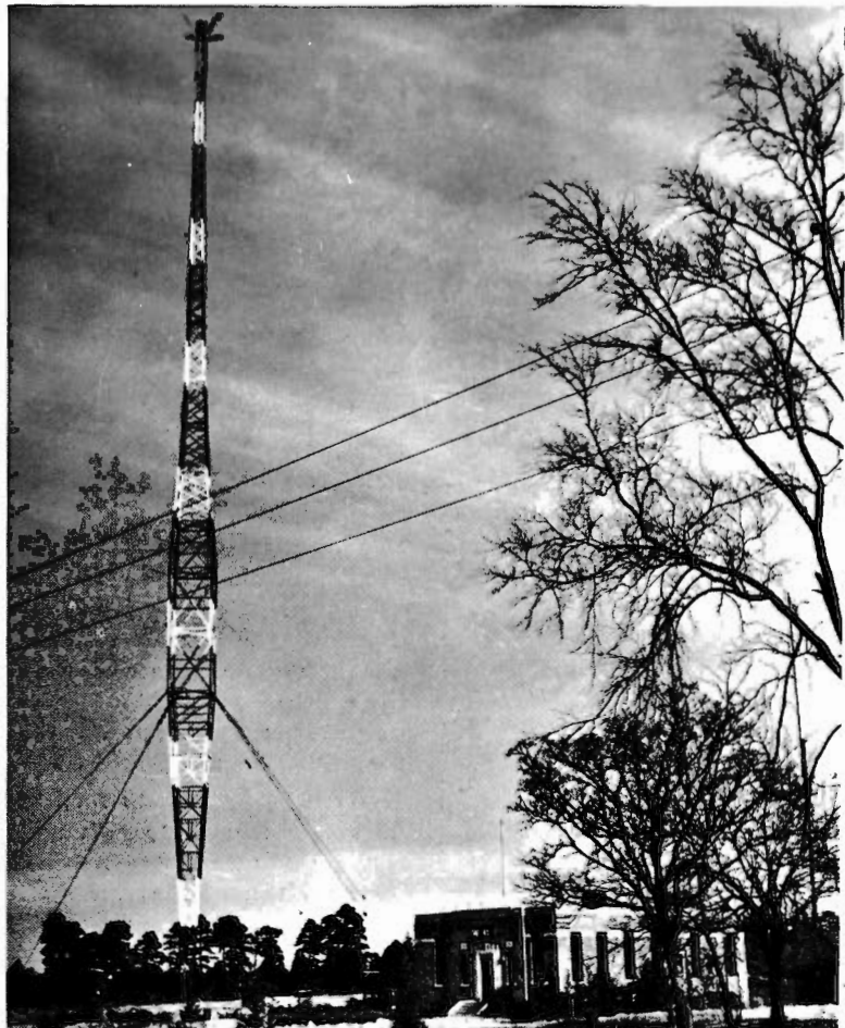
The New Vertical Radiator installed at Station WBT, Charlotte, N. C. This tower is 435 feet high
