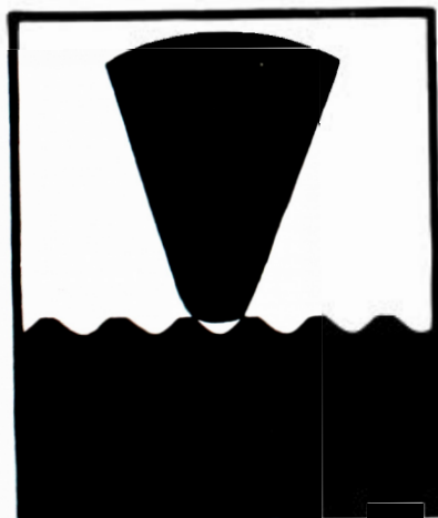
Needle C in standard groove before playing. (Note that needle rides the walls.)
