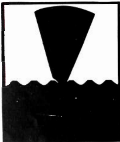
Needle A after playing a 16-inch record. (Note worn shoulder on groove.)
