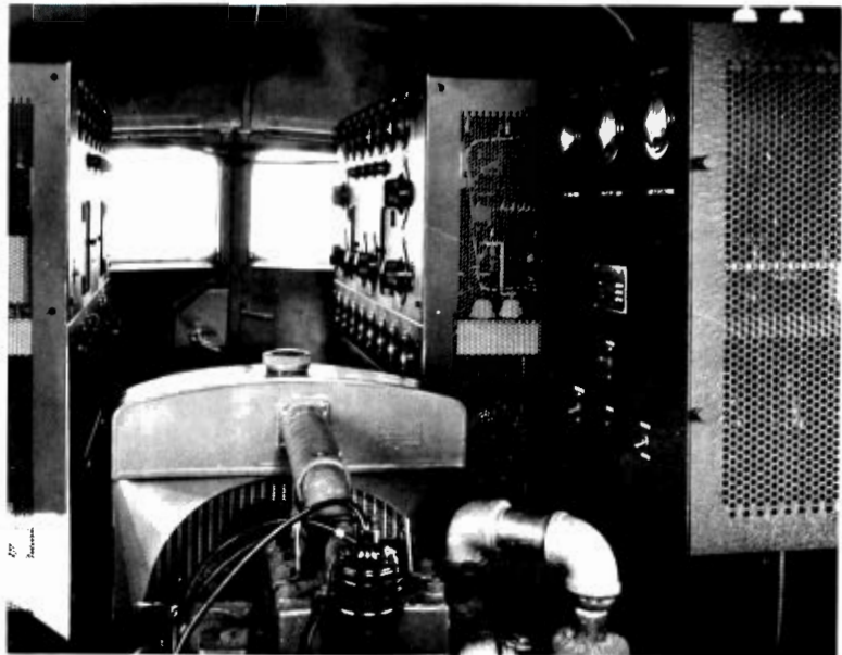
Showing the compact arrangement of equipment in the NBC Mobile Sound Unit.
