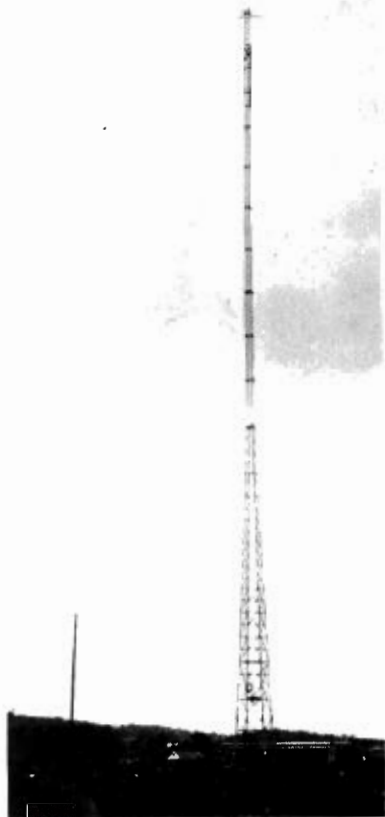
The new half-wave vertical radiator at WDOOD
