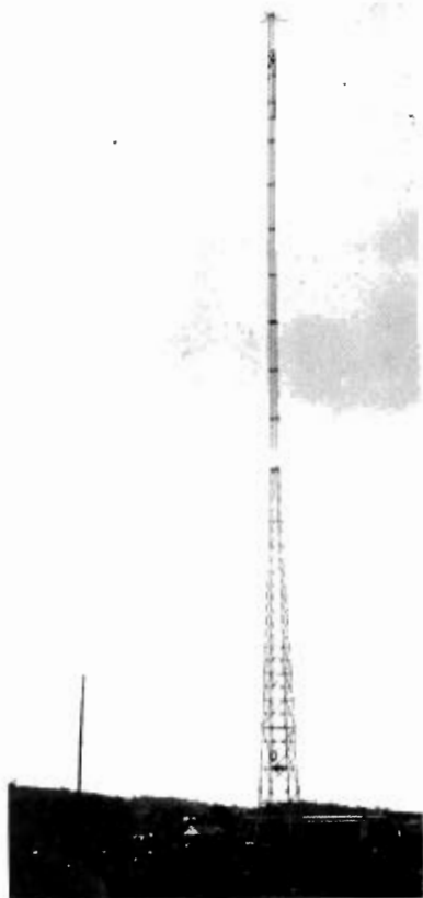
The new half-wave vertical radiator at WDOD
