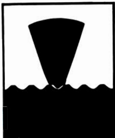
Needle C after playing a 16-inch record. (Emphasized shoulders wearing on both walls.)
