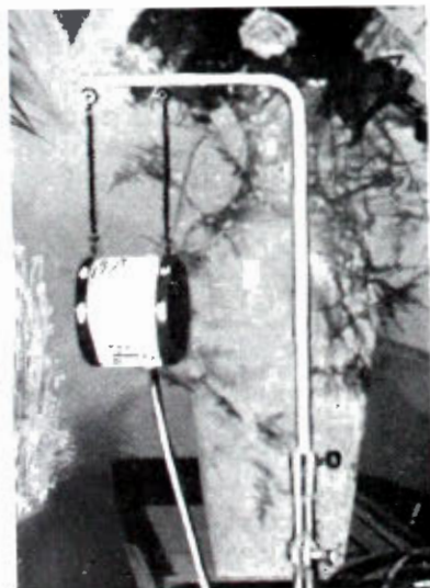
No. 3—The "Tomato Can" microphone, first used at stations KDKA and WJZ in 1922.
